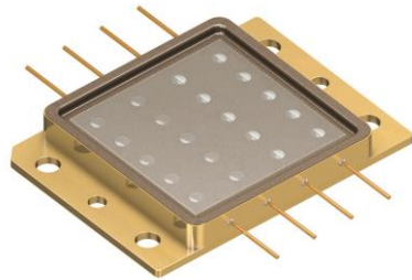
Figure 11 Matrice de 20 diodes LASER MARSO
