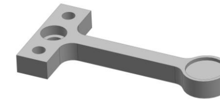
Figure 14 Pont support de miroir convexe
